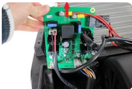
3) Slide out the PCB
