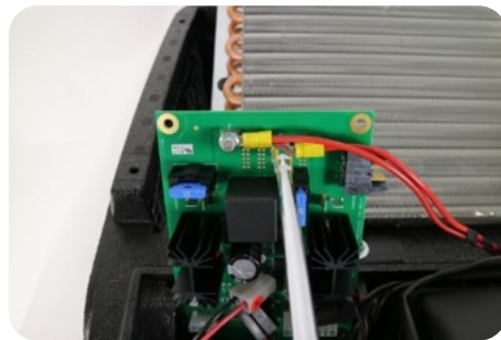
5) Unscrew the two compressor wire (2 nut-screw)
